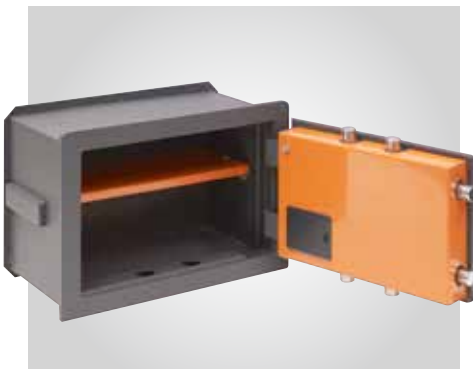
Rotary locking bolts avert any intent at cutting from the outside. Internal bolts housing.
